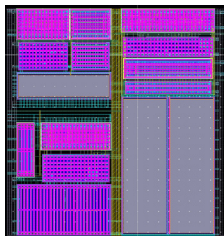
sAMP Cell Layout
